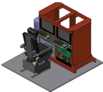
Wavefront Sensor Control Station
