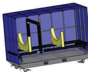
Pod Shipping Container with Cradle
