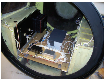
Radome Assembly
